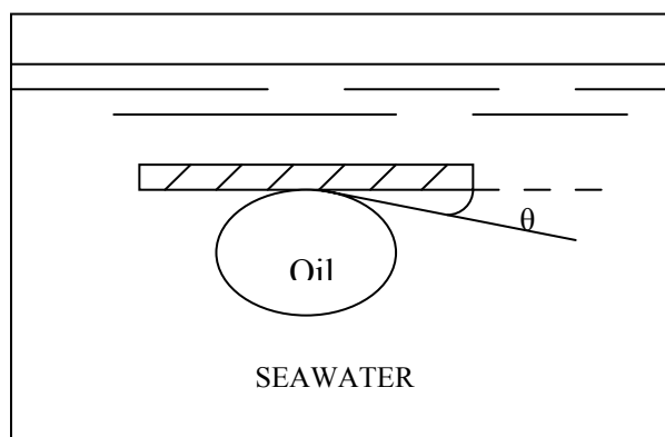
Figure 1. Illustration of phase arrangement in the cell for contact angle measurement
