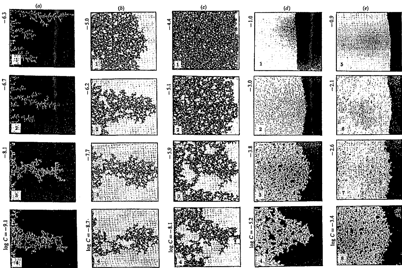
FIGURE 10. (a) Air (white) displacing a very viscous oil at various C at \log M = -4.7 : from viscous fingering (1) to capillary fingering (4). (b) Mercury (black) displacing hexane at \log M = 0.7 . (c) Mercury (black) displacing air at \log M = 1.9 . (d) Glucose solution (white) displacing oil at \log M = 2.0 and various C : from stable displacement towards capillary fingering. (e) Glucose solution (white) displacing oil at \log M = 2.0 and various C : from stable displacement towards capillary fingering.
