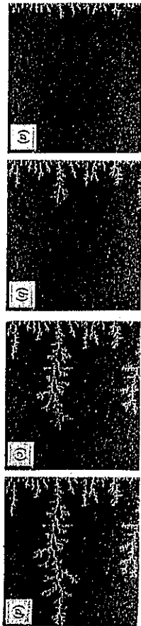
Figure 12. Different stages of the displacement of a very viscous oil by air.
