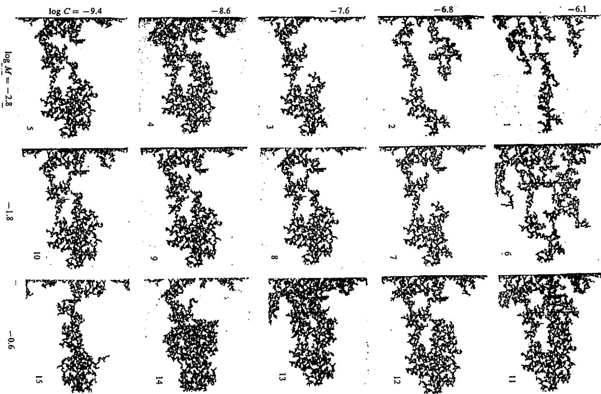
FIGURE 11. Mercury (black) displacing three various types of oils at different C and M . All the experiments are performed in the same micromodel.
