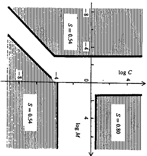
Figure 7. Plot of the constant-saturation domains for the 25 × 25 simulations.
