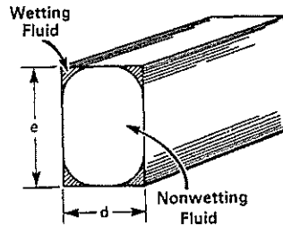
Figure 1. Situation of the fluids in a channel of the micromodel.
