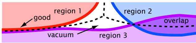
Figure 2: Each of the three regions is independently evolved in time, after which the interface locations do not agree. There are vacuums where all \phi_i are positive, and overlaps where more than one \phi_i is negative. The dotted black line shows the new interface locations after our projection step.
