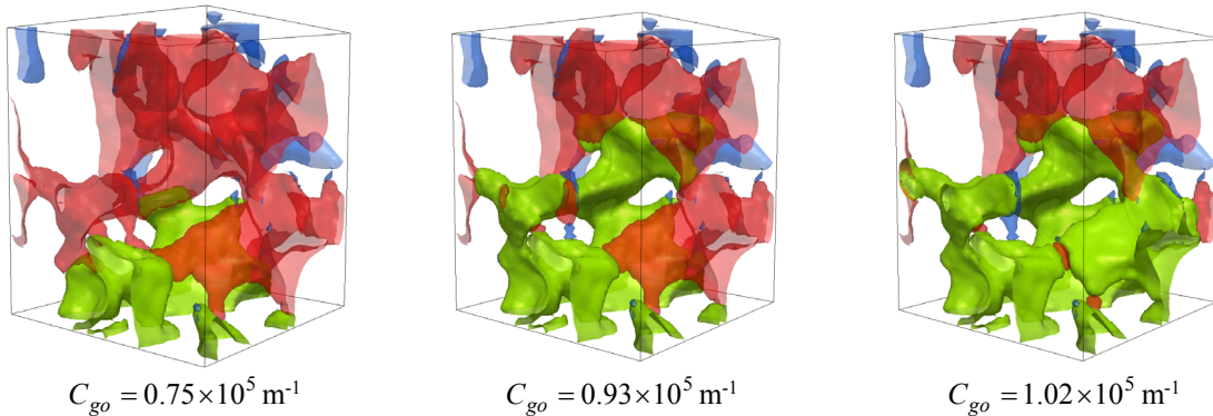
Figure 5: Stable fluid configurations of gas (green), oil (red) and water (blue) in Castlegate sandstone during gas invasion at constant oil-water capillary pressure from S_{wi} = 0.06 after primary drainage.
