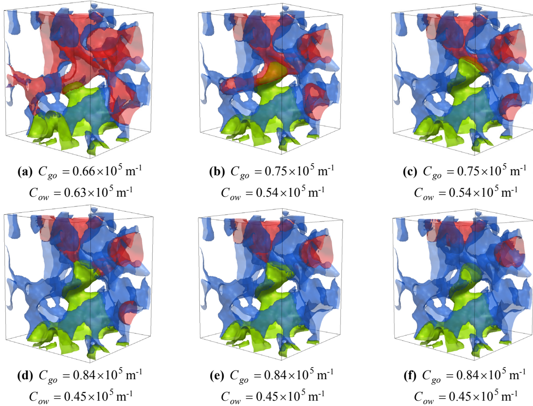
Figure 7: Stable (a, c and f) and unstable (b, d and e) three-phase configurations of gas (green), oil (red) and water (blue) in Castlegate sandstone for three combinations of gas-oil and oil-water capillary pressure during SWAG invasion from S_{wi} = 0.13 after primary drainage.
