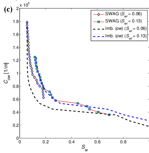
Figure 4: Simulation results in a pore structure extracted from a segmented three-dimensional image of Castlegate sandstone: (a) Displacement paths for gas invasion (G) and simultaneous water and gas invasion (SWAG) processes from two initial water saturations after two-phase oil/water primary drainage; (b) Three-phase gas-oil interface curvature as a function of total liquid saturation together with the two-phase oil/water primary drainage curve (PD); and (c) Three-phase oil-water interface curvature as a function of water saturation for the SWAG processes and the two-phase oil/water imbibition curves after primary drainage.
