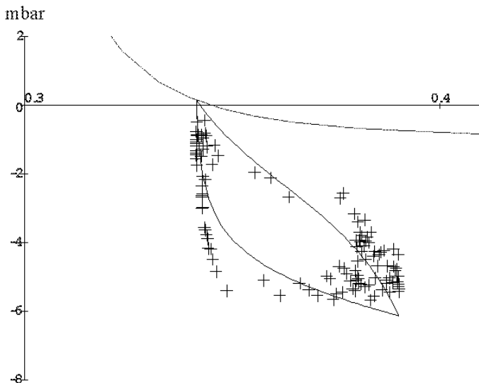
Fig. 11 Predicted small scanning loop and measured data.
