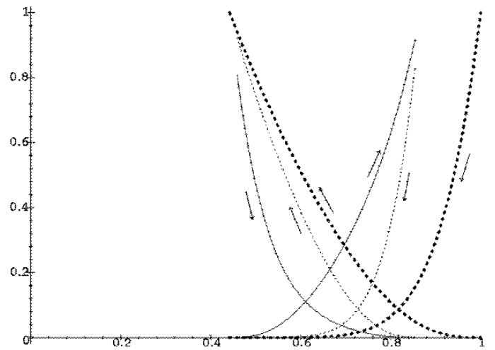
Fig. 20% Relative permeability curves for primary drainage, imbibition, and secondary drainage, data from Fig. 8.
