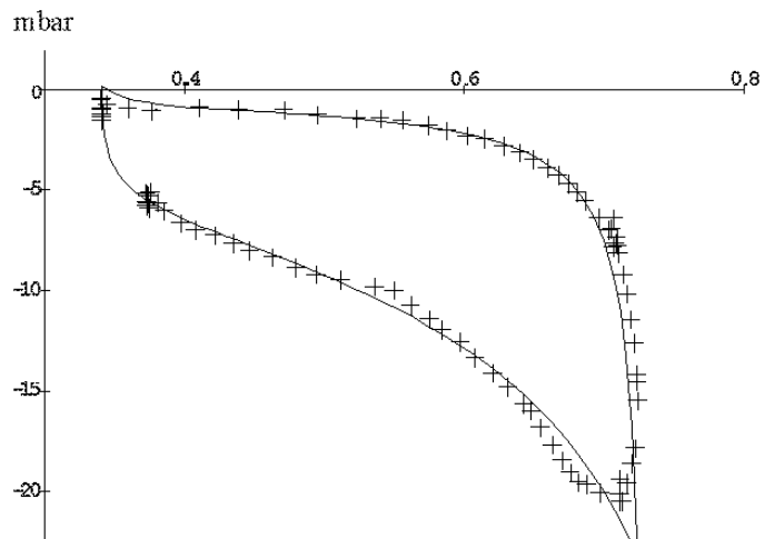
Fig. 9%Capillary pressure correlation fitted to the large scanning loop data.
