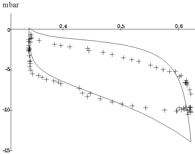
Fig. 10 Predicted medium scanning loop and measured data.
