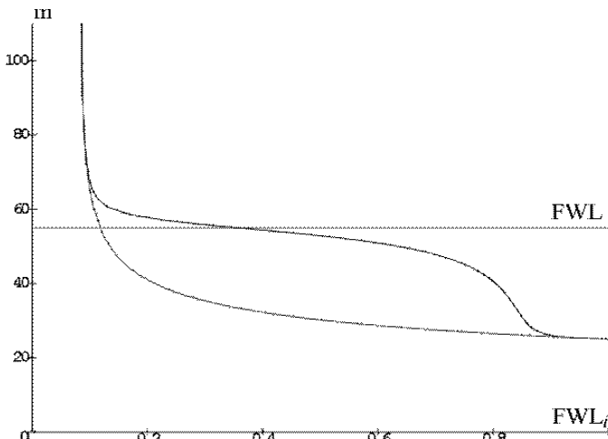
Fig. 6%Height above free water level (FWL) as a function of water saturation for two values of FWL; transition from a primary drainage curve at FWL, over to an imbibition dominated curve at FWL.
