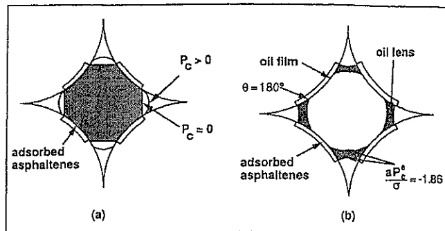
Figure 10. Imbibition processes in a mixed-oil-wet pore. (a) Spontaneous imbibition; (b) just after brine entry during forced imbibition.
