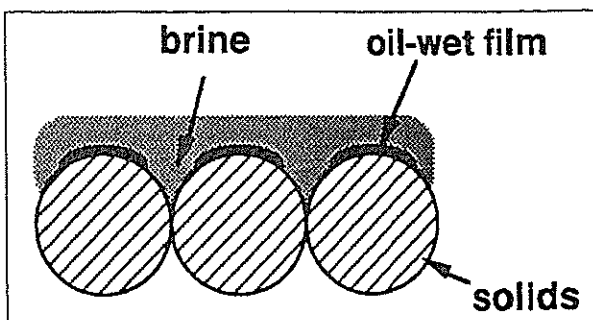
Figure 1. Mechanisms of oil surface drainage in mixed-wettability systems (after Salathiel, 1973).
