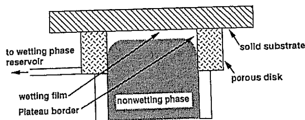
Figure 2. Apparatus for measuring thin-film forces in solid/liquid systems.
