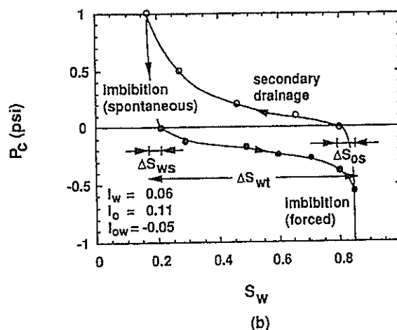
Figure 5. Typical experimental capillary pressure vs. aqueous-phase saturation curves.
