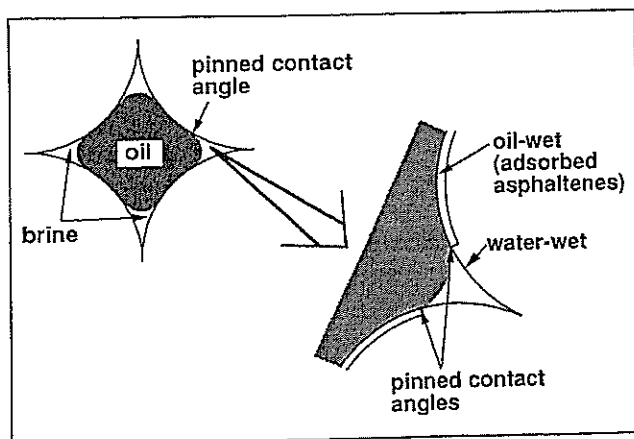
Figure 8. Mixed-oil-wet pore showing the location of asphaltene deposition and coexistence of oil-wet and water-wet regions within a single pore.
