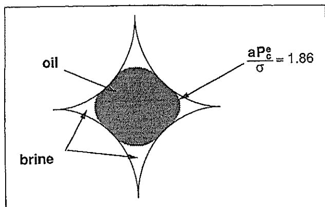
Figure 7. Water-wet pore just after oil entry.
