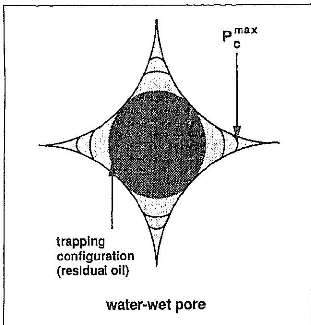
Figure 9. Imbibition processes in a water-wet pore.
