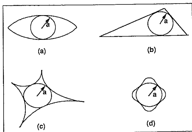
Figure 15. Alternative cross-sectional pore shapes.
