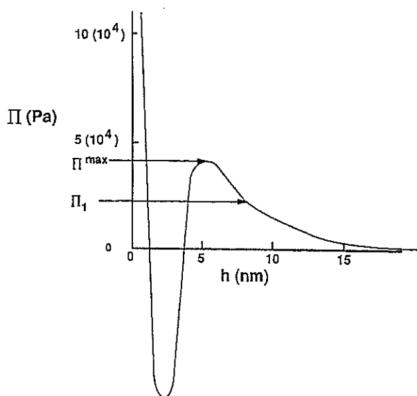
Figure 3. Disjoining pressure isotherm for wetting films on solids.
