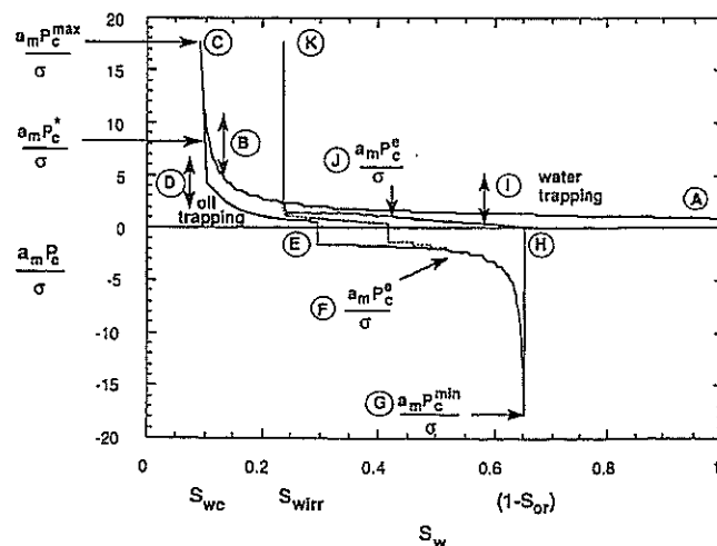
Figure 13. Capillary pressure vs. aqueous-phase saturation, case 1 unstable lenses.
