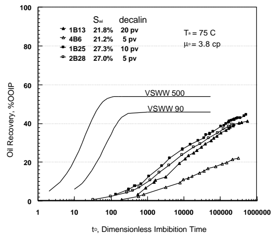
Figure 3. Sensitivity of MXW imbibition to decalin flush volume
