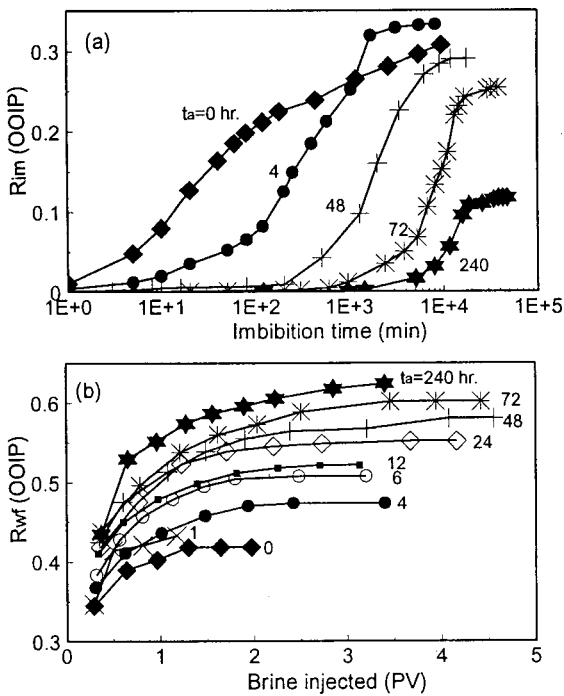
Fig. 2—(a) Oil recovery by imbibition vs. imbibition time and (b) oil recovery by waterflooding vs. pore volumes of brine injected for crude oil/brine/rock (COBR) systems at different aging times ( S_{wi}=15\% ).
