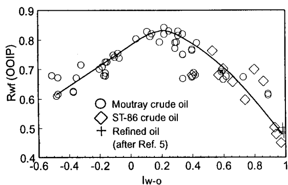
Fig. 1—Waterflooding recovery at 20 pore volumes (PV) of brine injection vs. Amott-Harvey wettability index for different oils.
