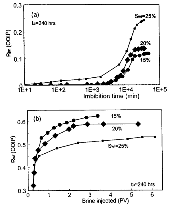
Fig. 5—Examples of the effect of initial water saturation on relationships between (a) oil recovery by imbibition vs. imbibition time and (b) oil recovery by waterflooding vs. PV of brine injected.
