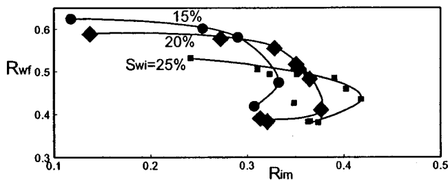
Fig. 6—Final waterflood oil recovery R_{wf} vs. final oil recovery by imbibition R_{im} for different initial water saturations.
