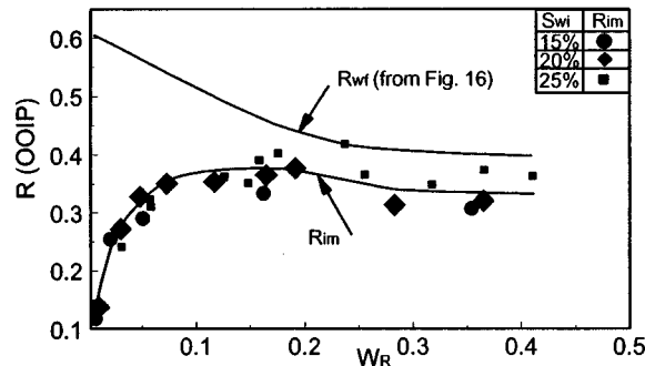
Fig. 17—Oil recovery by imbibition R_{im} and by final recovery R_{wf} vs. relative pseudowork of imbibition.
