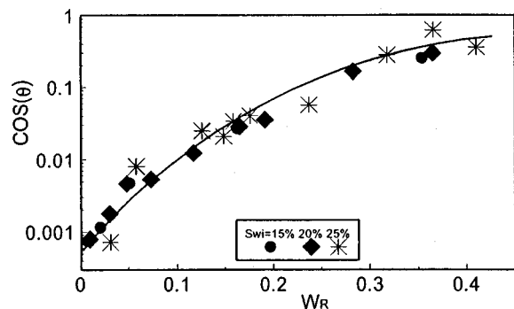
Fig. 12—Apparent dynamic advancing contact angle vs. relative pseudowork of imbibition.
