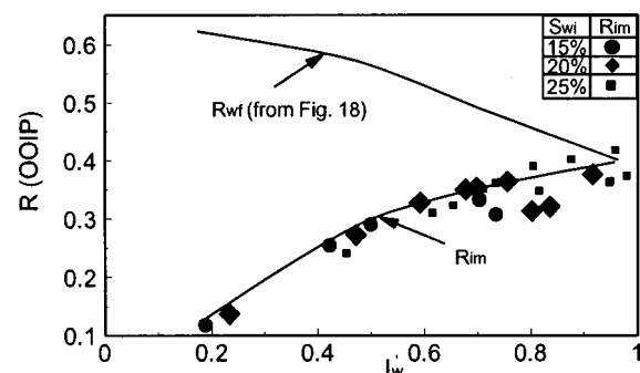
Fig. 19—Oil recovery by imbibition R_{im} and by waterflood R_{wf} vs. Amott wettability index to water.
