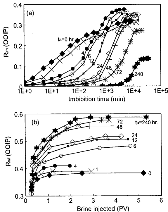
Fig. 3—(a) Oil recovery by imbibition vs. imbibition time and (b) oil recovery by waterflooding vs. pore volumes of brine injected for COBR systems at different aging times ( S_{wi}=20\% ).
