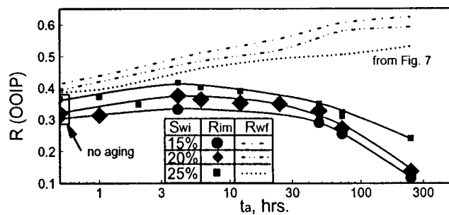
Fig. 8—Final oil recovery by imbibition R_{im} and final waterflood oil recovery R_{wf} vs. aging time at different initial water saturations.
