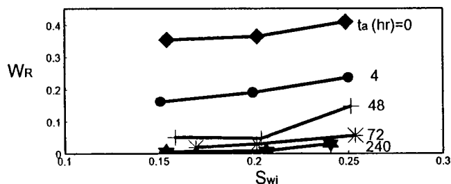
Fig. 14—Effect of aging time on relationships between initial water saturation and relative pseudowork of imbibition.
