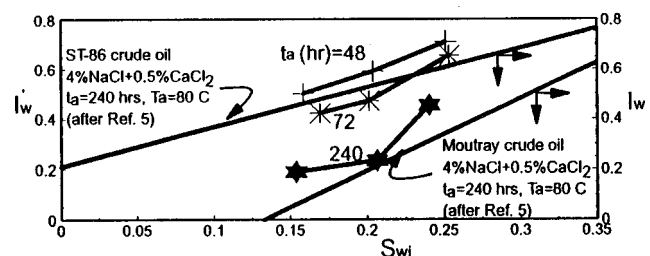
Fig. 15—Comparison of relationships between S_{wi} and I'_w with different COBR systems.
