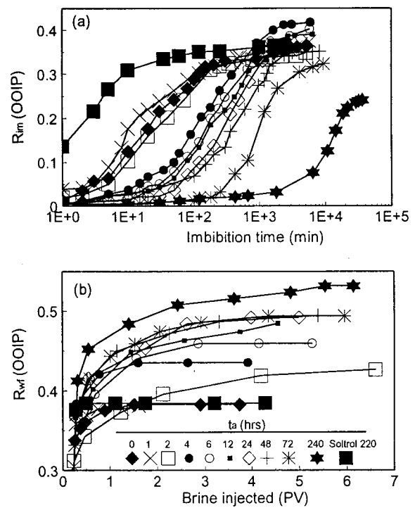
Fig. 4—(a) Oil recovery by imbibition vs. imbibition time and (b) oil recovery by waterflooding vs. pore volumes of brine injected for COBR systems at different aging times ( S_{wi}=25\% ).
