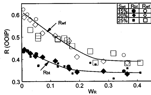
Fig. 16—Oil recovery by waterflooding at breakthrough R_{bt} and final recovery R_{wf} vs. relative pseudowork of imbibition.
