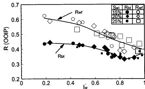
Fig. 18—Oil recovery by waterflooding at breakthrough R_{bt} and final recovery R_{wf} vs. Amott wettability index to water.
