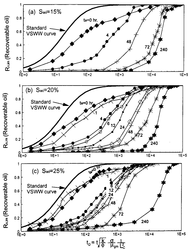
Fig. 9—Effect of aging time on relationships between normalized oil recovery by imbibition and dimensionless time for systems with nominal initial water saturations of (a) 15%, (b) 20%, and (c) 25%.
