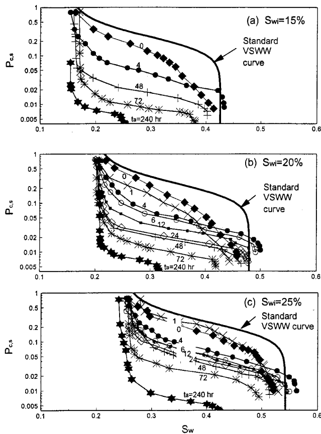
Fig. 10—Effect of aging time on pseudocapillary pressure curves for systems with initial water saturations of (a) 15%, (b) 20%, and (c) 25%.
