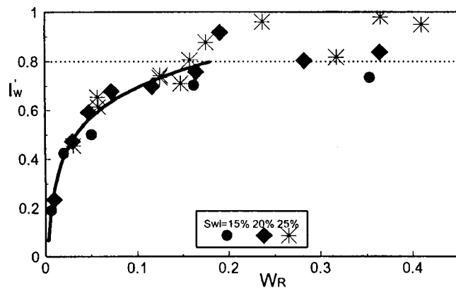
Fig. 11—Amott wettability index to water I'_w vs. relative pseudowork of imbibition W_R .
