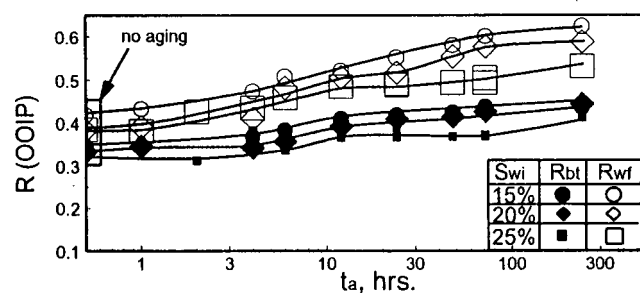
Fig. 7—Oil recovery by waterflooding at breakthrough R_{bt} and final waterflood oil recovery R_{wf} vs. aging time at initial water saturations of 15, 20, and 25%.
