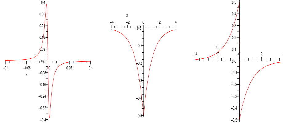
FIGURE 2. Plot of kernels corresponding to Left: well-reservoir model G_1(x) ; Middle: Burger Poisson G_2(x) , Right: radiating gas G_3(x) .
