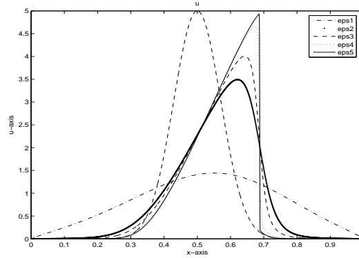
FIGURE 3. Plot of solutions at time T = 0.02 with r = 10^{-4} for different choices of \varepsilon corresponding to \varepsilon_1 = 10^7 , \varepsilon_2 = 10^6 , \varepsilon_3 = 5 \cdot 10^5 , \varepsilon_4 = 10^5 , and \varepsilon_5 = 0 . Loss of regularity is seen for \varepsilon > 0 .
