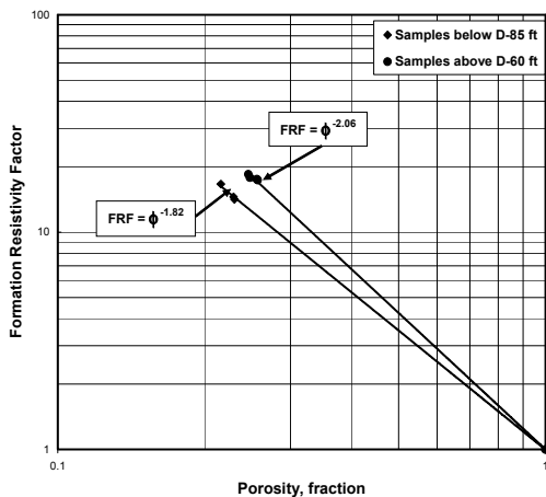
Figure 1. Interval Avg. Formation Resistivity Factor.
