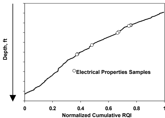
Figure 3. Cumulative RQI Plot.
