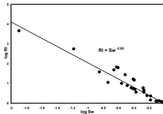
Figure 2. Composite Resistivity Index.
