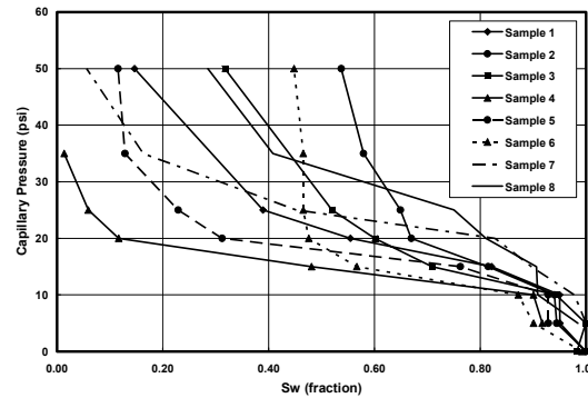
Figure 4. Capillary Pressure Curves.
