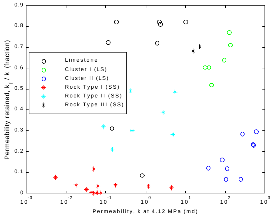
Figure 10: Permeability retained versus laboratory determined permeability at an effective confining pressure of 4.12 MPa.
