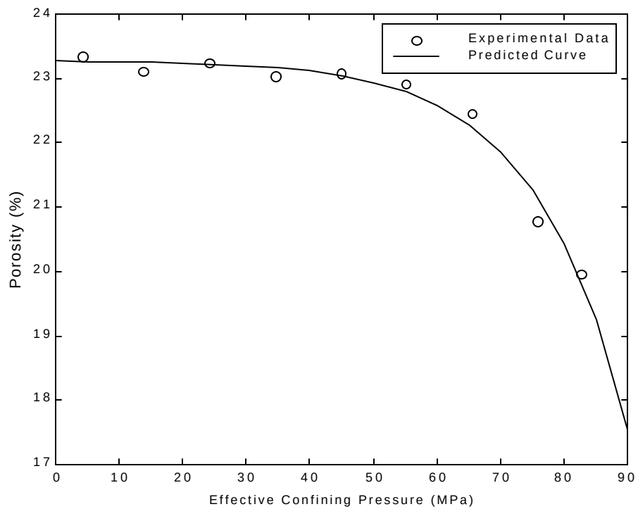
Figure 4: Porosity versus effective confining pressure curve with curve fit for a representative reservoir limestone sample.
