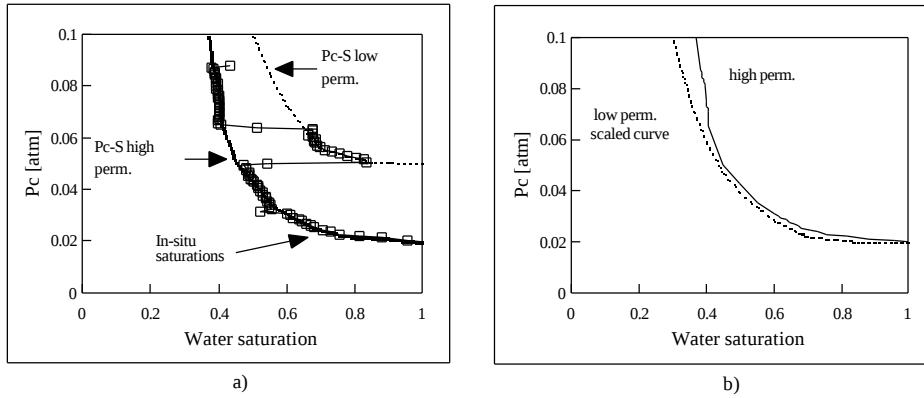
Figure 6. Equilibrium calculations of P_c -S from in-situ saturation measurements. The capillary pressure as function of saturation is calculated by knowing the height above FWL and assuming equilibrium between gravity and capillary forces (a) . The low permeability capillary pressure curve is scaled with permeability and porosity to the analogue values of the high permeability curves (J-function approach). Agreement between the capillary pressure for low and high permeability Berea is obtained (b) .
