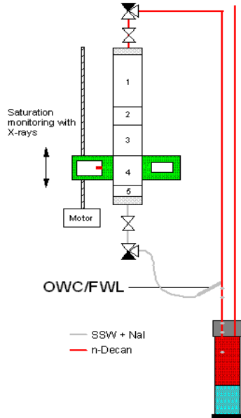
Figure 2. Experimental set-up
