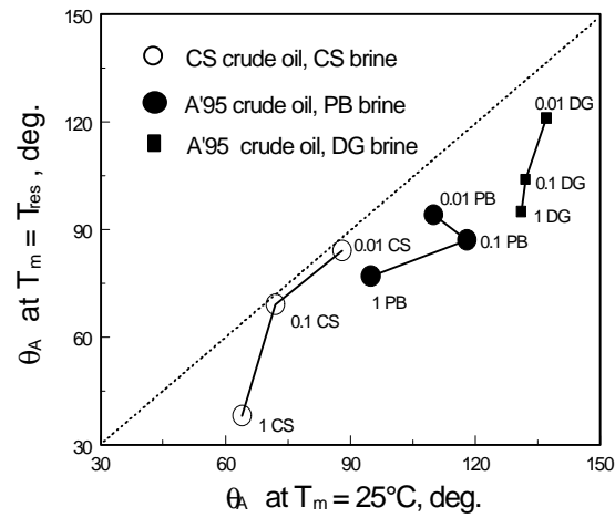
Fig. 5 The effect of temperature of measurement on advancing angles.
