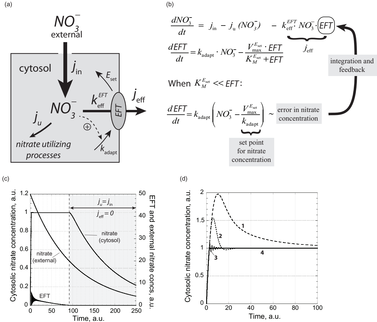
Figure 4. Representation of outflow controller motif (Fig. 3). (a) External nitrate flows into the cytosol by flux j_{in} . Nitrate is utilized within the cytosol by various processes, which are described by nitrate-removing flux j_u . EFT is a nitrate-inducible efflux transporter, pumping nitrate out of the cell with flux j_{eff} . (b) Kinetic representation of outflow controller in (a). Fluxes j_{in} and j_u may fluctuate with time. To maintain homeostasis j_{in} needs to be larger than j_u . The rate dEFT/dt is proportional to the error between nitrate concentration and its set point, while EFT (corresponding to E in Figs 2 & 3) represents the integrated error. (c) Model calculation of homeostatic behaviour. Flux j_{in} decreases by a first-order process j_{in}(t) = (NO_{external}^-)_0 \cdot e^{-0.01t} with the initial value of the external nitrate concentration as (NO_{external}^-)_0 = 50 a.u. The nitrate utilizing flux is also considered to be a first-order process, i.e. j_u = 0.2 \cdot (NO_3^-) . The other parameter values are: k_{adapt} = V_{max}^{E_{set}} = 1.0 \times 10^6 a.u. giving a set point of 1, k_{eff}^{EFT} = 0.1 and K_M^{E_{set}} = 1.0 \times 10^{-9} . Initial concentrations in NO_3^- and EFT are both 0. (d) An increased k_{adapt} (gain) leads to increased aggressiveness of the controller, i.e. the homeostatic set point is more rapidly approached during a perturbation with increased aggressiveness. To keep the homeostatic set point constant V_{max}^{E_{set}} is increased together with k_{adapt} . Curves 1–4 show approaches to the homeostatic set point with the following k_{adapt} = V_{max}^{E_{set}} values (in a.u.): 1, 0.1; 2, 1.0; 3, 1.0 \times 10^2 ; 4, 1.0 \times 10^5 . Initial concentrations (in a.u.): external nitrate concentration is 50.0, while initial cytosolic nitrate and EFT concentrations are 0. For the sake of simplicity, the external nitrate concentration in this set of calculations is kept constant.
