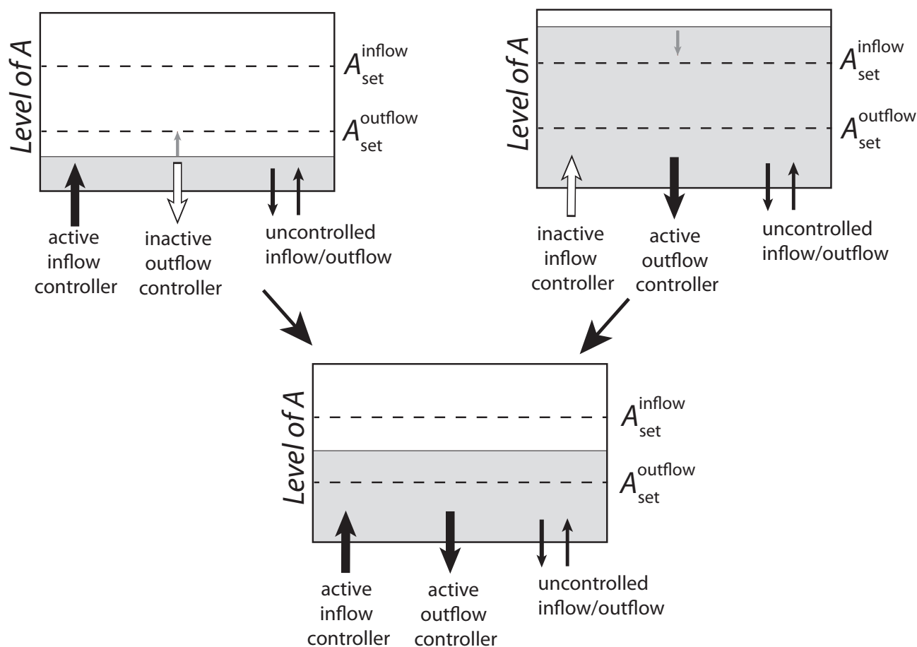
Figure 7. Behaviour of cooperative inflow and outflow controllers when A_{set}^{outflow} < A_{set}^{inflow} . In this case, independent of initial A levels and dominance of uncontrolled inflow/outflow conditions to and from A , both controllers are active and steady state values of A end up between A_{set}^{inflow} and A_{set}^{outflow} dependent on the aggressiveness of the individual controllers. E levels for each controller may steadily increase in this case a situation termed as integral wind-up.
