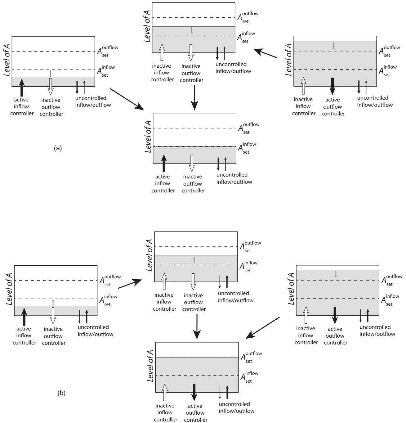
Figure 6. Behaviour of cooperative inflow and outflow controllers when A_{set}^{outflow} > A_{set}^{inflow} . (a) Uncontrolled removal/outflow of A is dominant. Large white arrows indicate an idle/inactive controller, while large black arrows indicate an operating/active controller. Left: when initial levels of A are below A_{set}^{inflow} inflow controller is active and outflow controller is inactive. A levels are regulated to the set point A_{set}^{inflow} . Right: when initial levels of A are above A_{set}^{outflow} the outflow controller is active while the inflow controller is inactive. Middle: the uncontrolled (dominating) outflow drives A levels below A_{set}^{outflow} and both controllers are inactive. Once A levels fall below A_{set}^{inflow} , the inflow controller becomes active and keeps A at A_{set}^{inflow} . (b) Uncontrolled addition/inflow of A is dominant. Left: when initial levels of A are below A_{set}^{inflow} inflow controller is active and outflow controller is inactive. Middle: when A level is above A_{set}^{inflow} , both controllers are idle and A increases. Once A levels are above A_{set}^{outflow} , the outflow controller becomes active and keeps A at A_{set}^{outflow} . Right: when initial levels of A are above A_{set}^{outflow} the outflow controller is active and keeps A at A_{set}^{outflow} . In case the uncontrolled inflow and outflow rate to and from A are precisely the same (not shown), final A levels are kept either at A_{set}^{inflow} when initial A value is lower than A_{set}^{outflow} , or at A_{set}^{outflow} when initial A value is higher than A_{set}^{outflow} . In case initial A level lies between A_{set}^{inflow} and A_{set}^{outflow} , none of the controllers are active and no change in A occurs.
